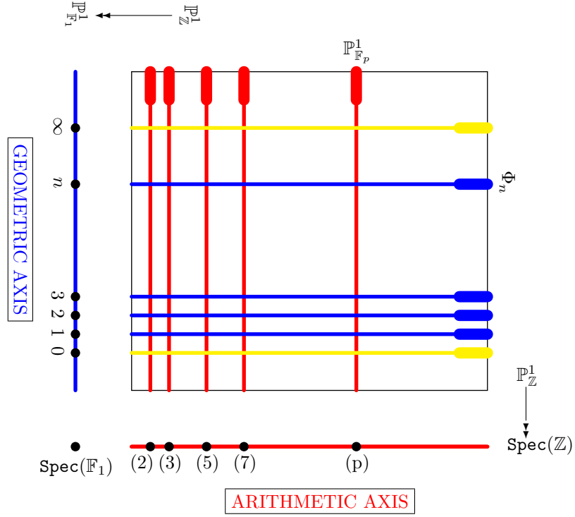
Figure 1. The extended Mumford drawing
