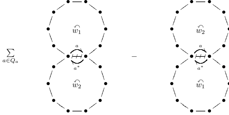
FIGURE 1. Lie bracket [w_1, w_2] in \mathfrak{N}_Q .
